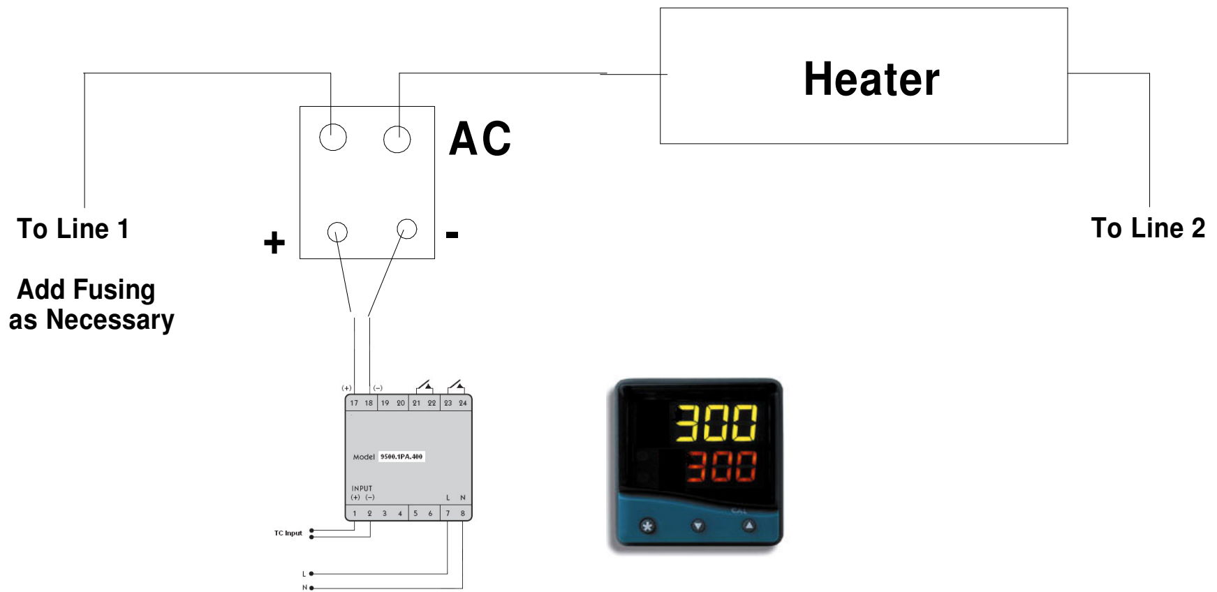
CAL 9500 Temperature Controller
